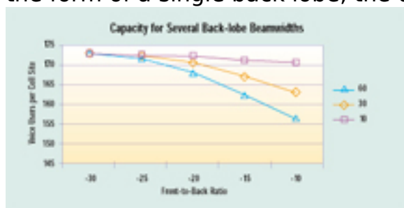
Figure 6. Capacity predictions for a typical three sector cell site configuration rotated by 30 degrees. The different lines are for the back-lobe beamwidths 60, 30 and 10 degrees.
