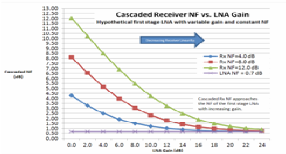
Figure 2: Plot of Cascaded NF vs. LNA Gain
