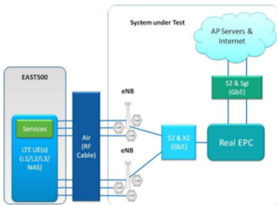
LTE network architecture
